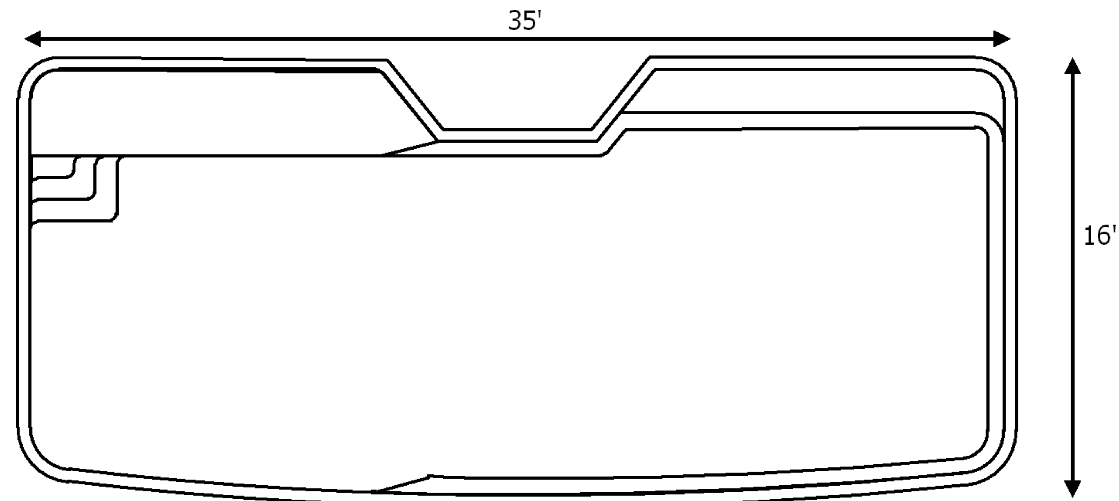
Outside Dimensions
